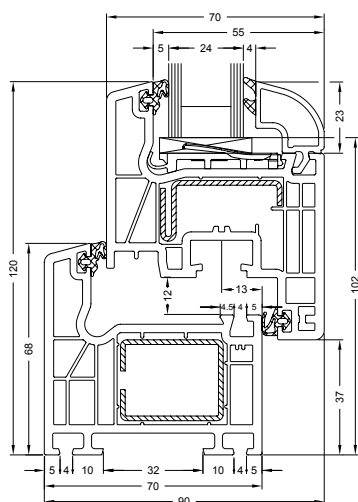
Schüco Corona CT 70 AS Classic
